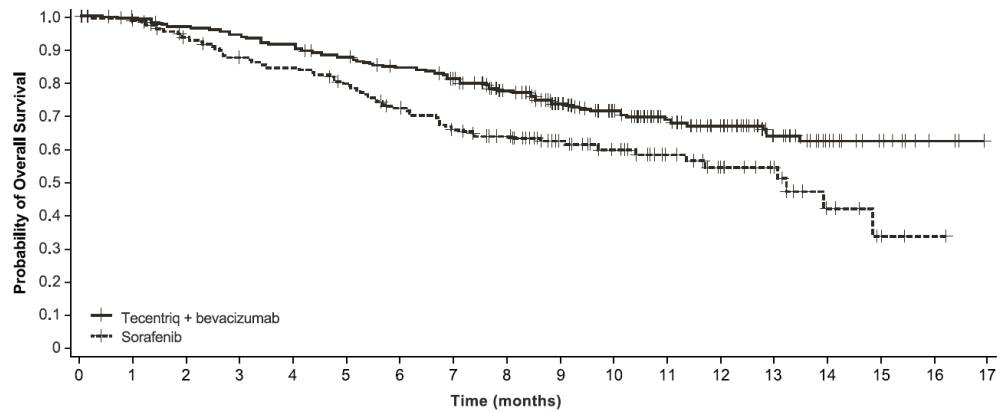
Figure 18: Kaplan-Meier Plot for Overall Survival (IMbrave150)
