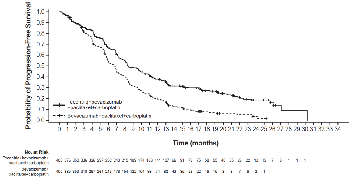
Figure 4: Kaplan-Meier Plot for updated Progression Free Survival in the ITT population (IMpower150)
