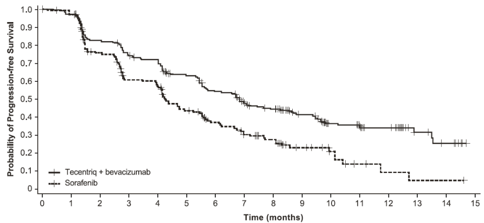
Figure 19: Kaplan-Meier Plot for Progression-Free Survival per RECIST v1.1 (IMbrave150)
